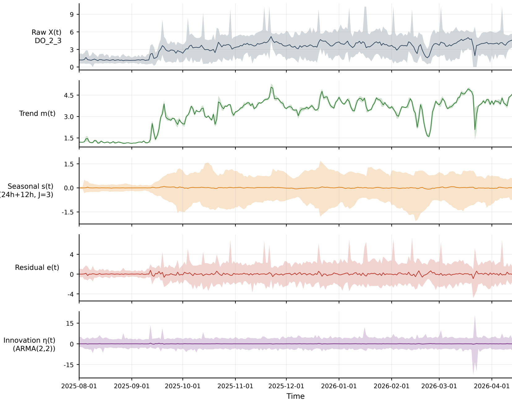
Full-span daily overview — DO_2_3 (aerobic, min) [2025-08-01~2026-04-13]
